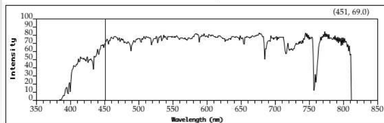
Electromagnetic Spectrum
